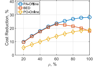
Fig. 5. Cost reduction vs different local capacities.
