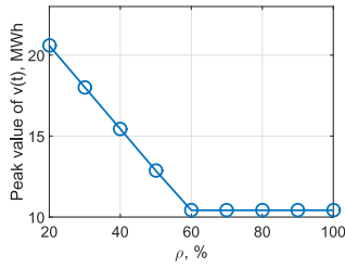
Fig. 6. \max v(t) of PA-Offline vs \rho .
