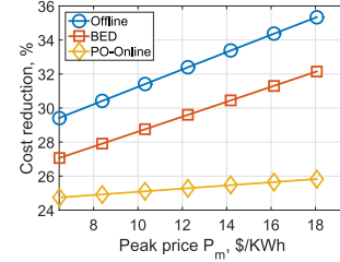
Fig. 8. Cost reduction with different peak price on a small microgrid testbed.
