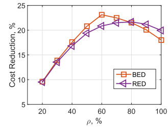
Fig. 7. Comparison of RED and BED under different local capacities.
