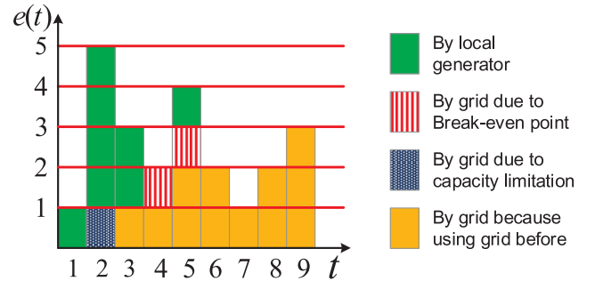
Fig. 2. Demonstration of BED with C = 4 , different colors denoting different strategies of the algorithm.
